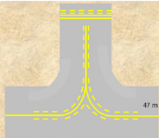
Enhanced taxi guideline at "T" intersection (Illustration)
