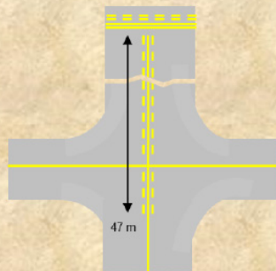
Enhanced taxi guideline at cross intersection (Illustration)
