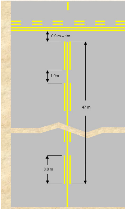
Enhanced taxi guideline at cross intersection (Illustration)
